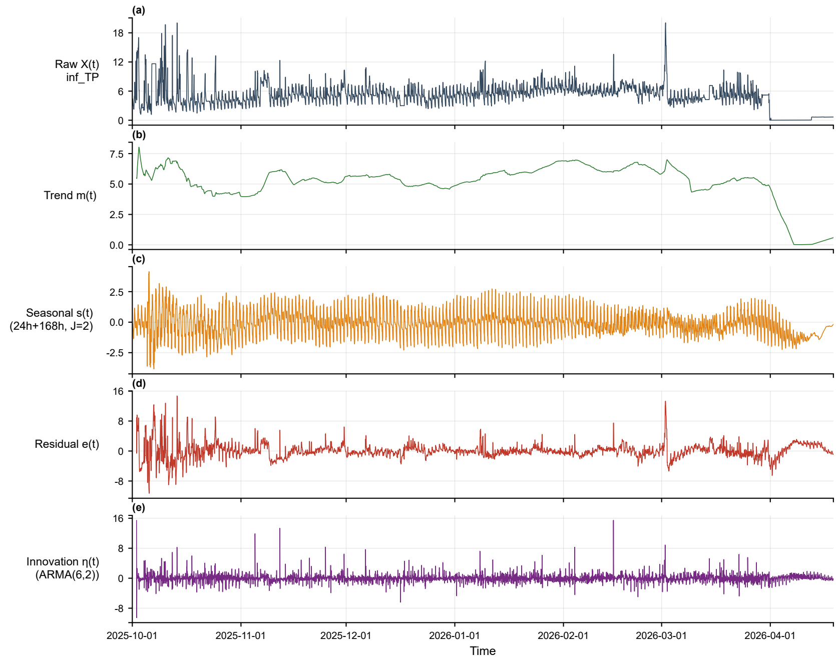
Multi-scale decomposition — inf_TP (influent, hour) [2025-10-01~2026-04-19]
